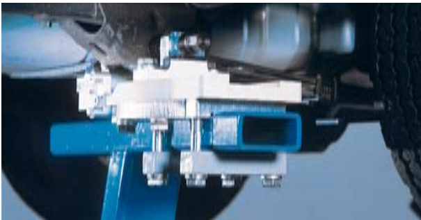
B260 clamp holds tightly to the spring shackle without removing the spring. Saves time and expense.
