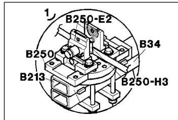
Line drawings on data sheets show exactly how and where to mount the clamps.
